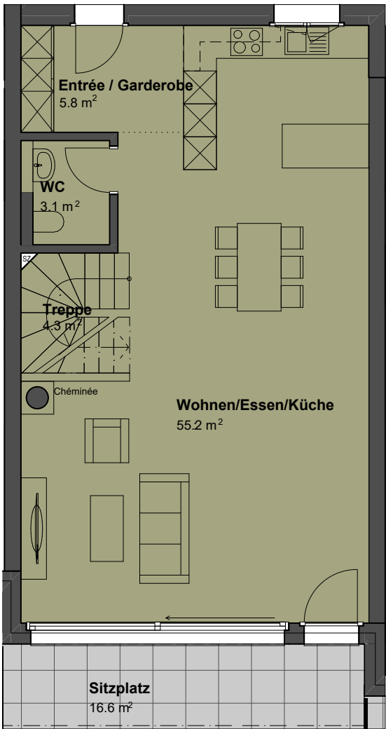
Erdgeschoss 69.2 m²
