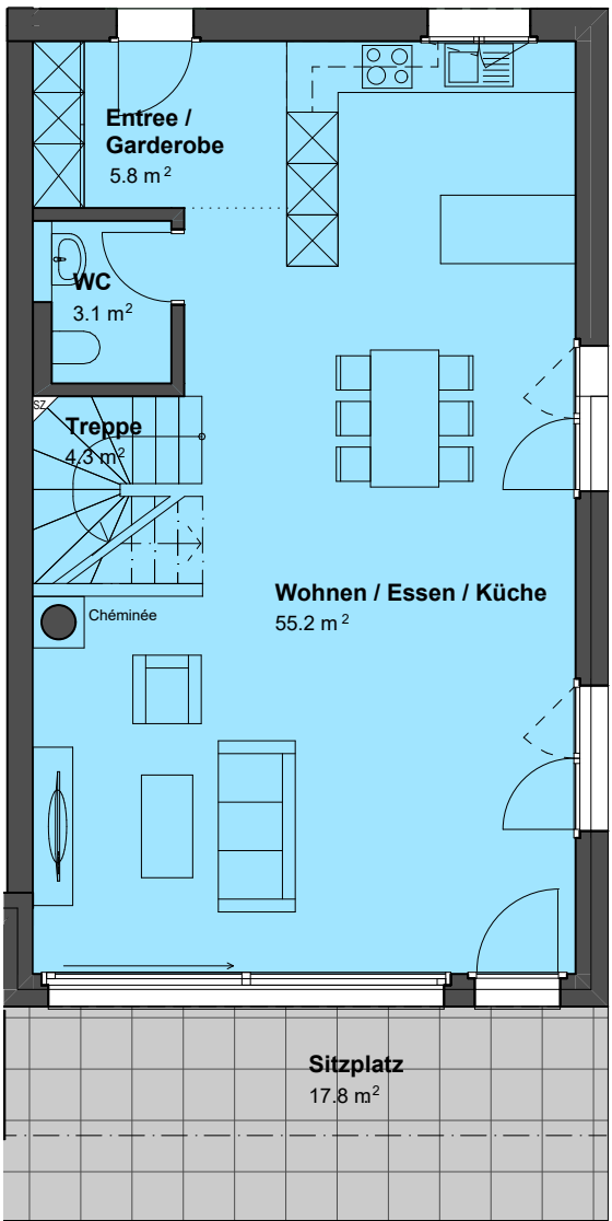
Erdgeschoss 69.2 m²
