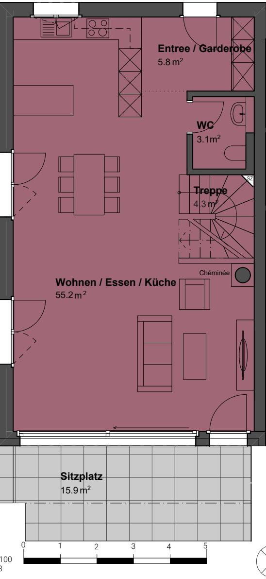
Erdgeschoss 69.2 m²
